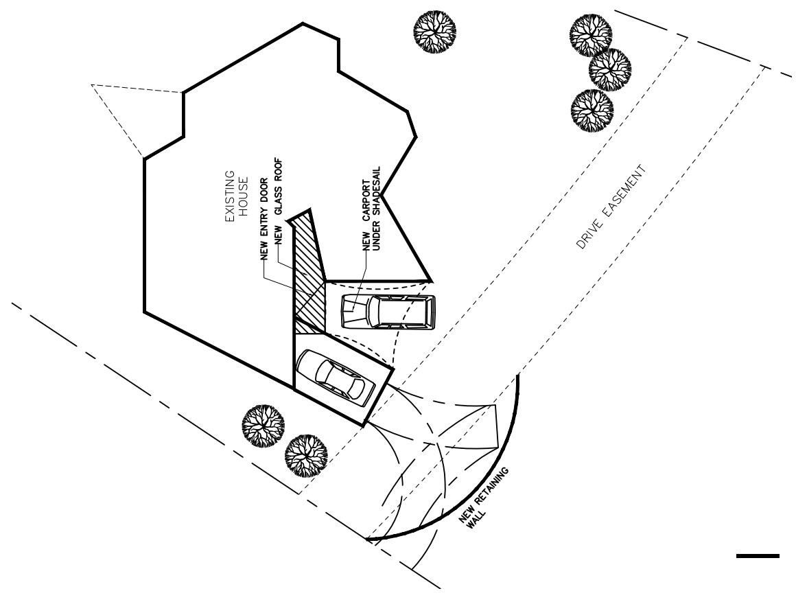
2-CAR GARAGE INTO HILLSIDE, 15' HIGH RETAINING WALLS
